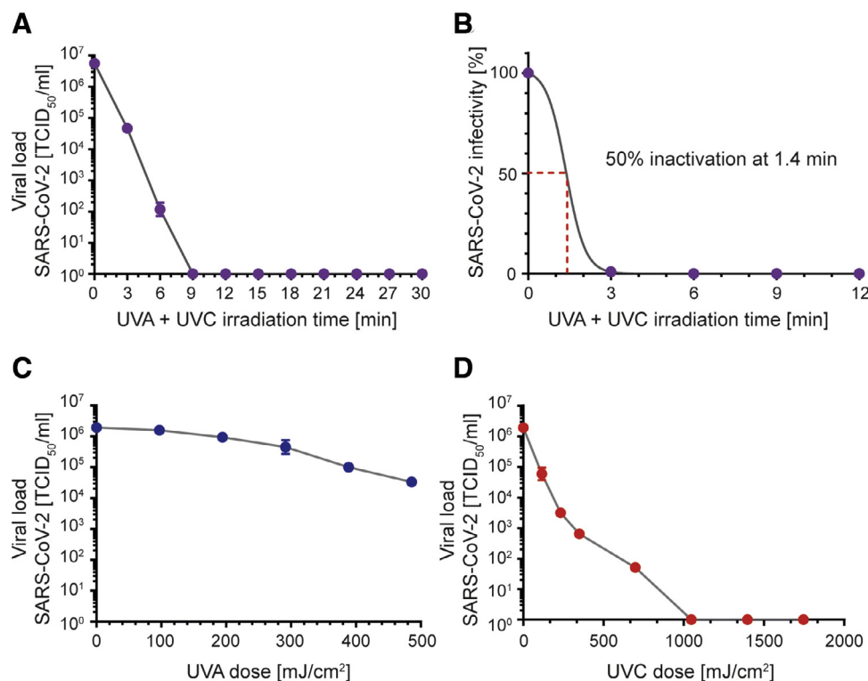
Fig 1. Inactivation of SARS-CoV-2 by UV irradiation. SARS-CoV-2 at a starting concentration of 5 \times 10^6 \text{ TCID}_{50}/\text{mL} was irradiated with ultraviolet light (UV). UV treatment was performed by irradiation with UVC (254 nm) and/or UVA (365 nm) on 600 \mu\text{L} aliquots of virus in 24-well plates. The UV light source was placed at a distance of 3 cm above the bottom of the plate. Viral loads were determined by end point dilution after (A) combined UVA/UVC exposure at the indicated time points or separate exposure to (C) UVA light after 0, 3, 6, 9, 12, and 15 minutes or (D) UVC light after 0, 1, 2, 3, 6, 9, 12, and 15 minutes. (B) Nonlinear regression was conducted to calculate the duration of combined UVA and UVC irradiation sufficient to inactivate the virus by 50%. The emitted light dose was measured with = 1940 \mu\text{W}/\text{cm}^2 for UVC (254 nm) and 540 \mu\text{W}/\text{cm}^2 for UVA (365 nm) at a distance of 3 cm. This corresponds to an applied light dose of 1.94 \text{mJ}/\text{cm}^2 per second for UVC and 0.54 \text{mJ}/\text{cm}^2 per second for UVA ( \mu\text{W} = 10^{-6} \text{ J/s} ). The experiments were performed in triplicates. Error bars represent the standard deviation of the mean.
